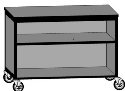
-1220 25D x 48W x 36H 1 Adjustable Shelf
